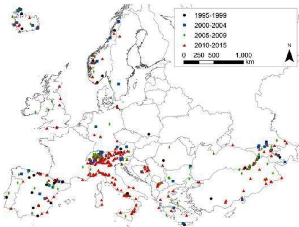
Figure 3.3. Spatial distribution of fatal (death, injury, and missing) landslides in the European Continent from 1995 to 2015.
